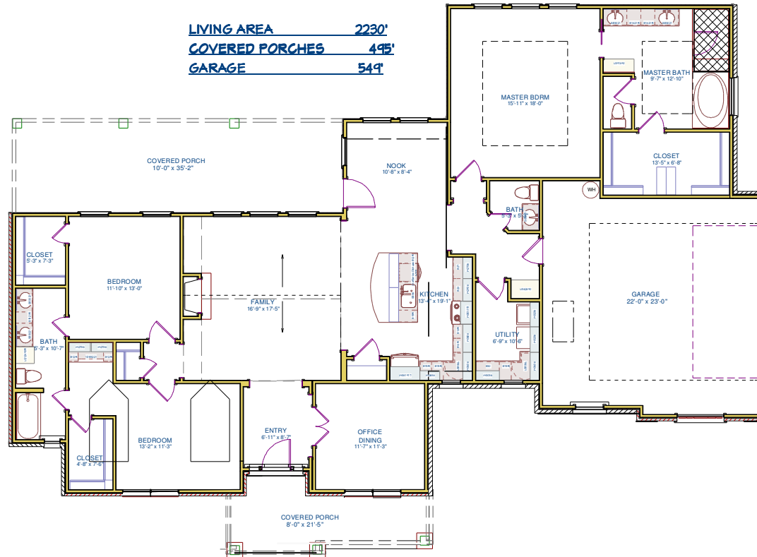
FLOOR PLAN
