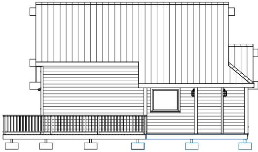
LEFT ELEVATION
